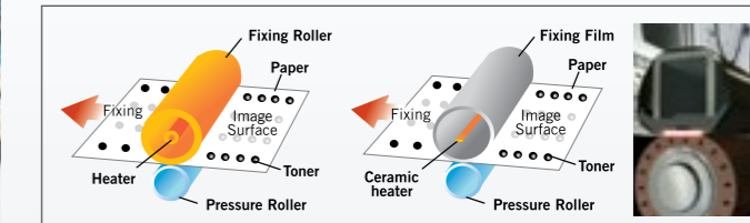
Conventional Roller Fixing Method
